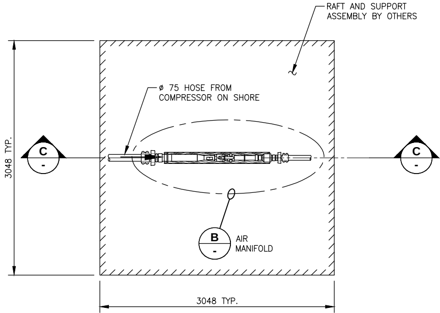
A PLAN - DIFFUSER RAFT SCALE 1:50
