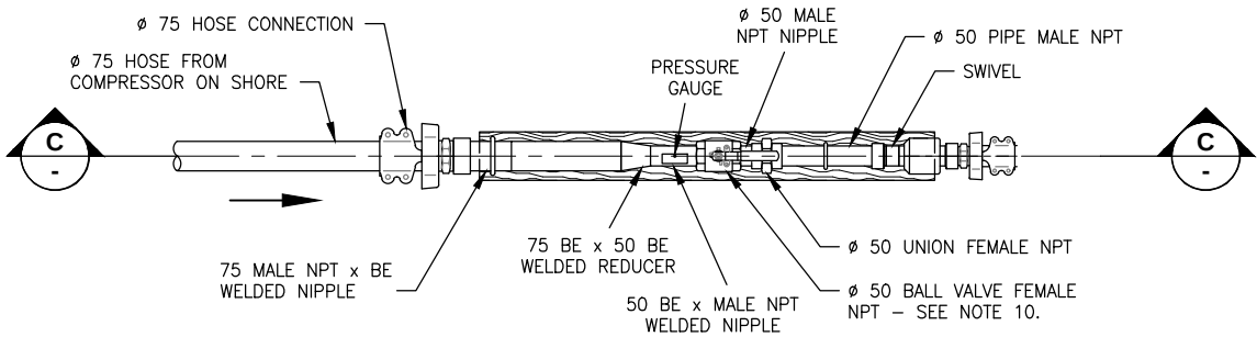
B PLAN - AIR MANIFOLD SCALE 1:25
