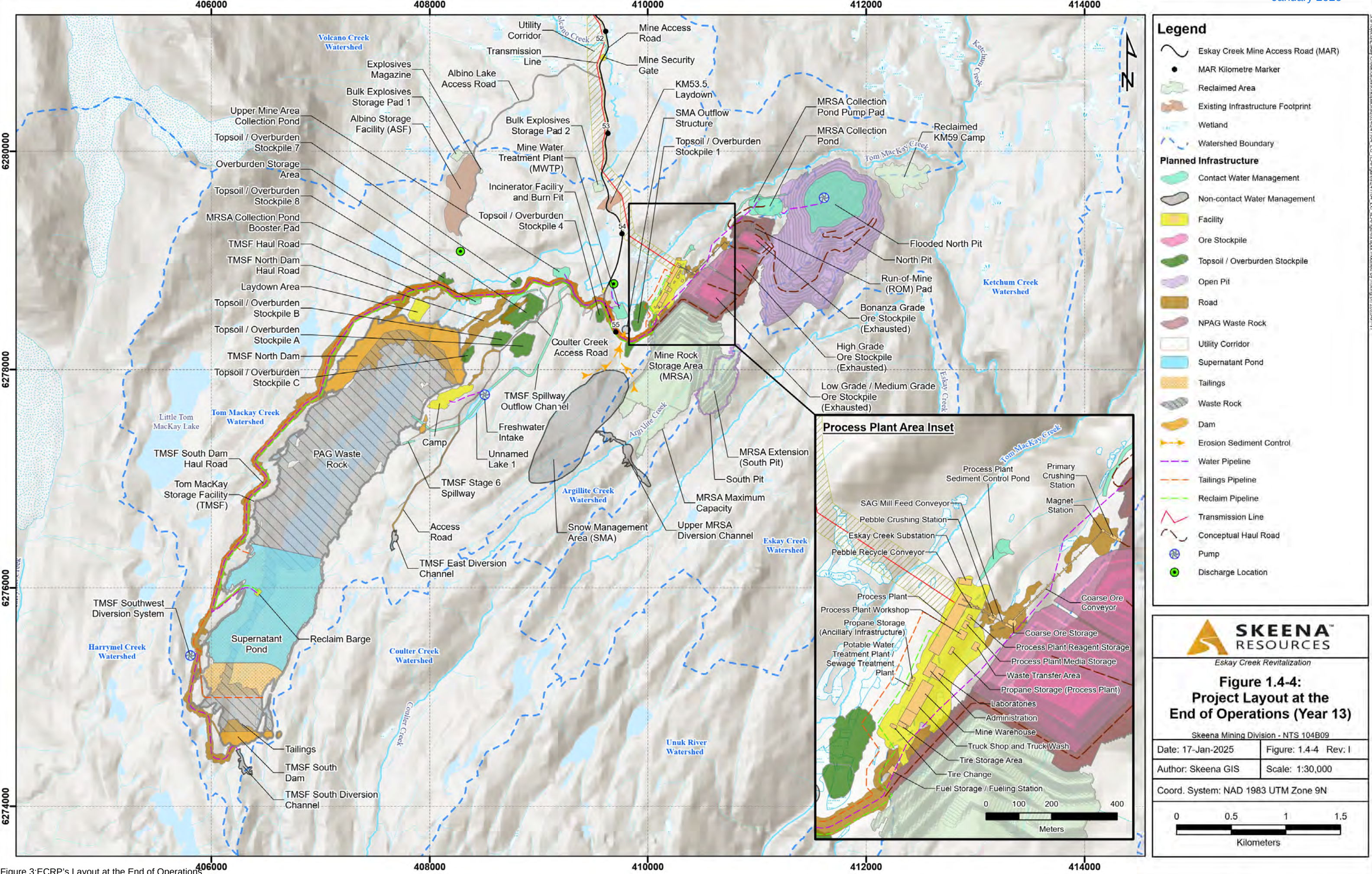
Figure 3: ECRP's Layout at the End of Operations
